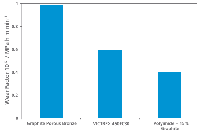
Figure 27: Wear Factor at 200°C (390°F), with 3 \text{ m s}^{-1} (600 ft \text{min}^{-1} ) and 20 kg (44 lb) Load for some of the Highest Tribological Performance Materials
