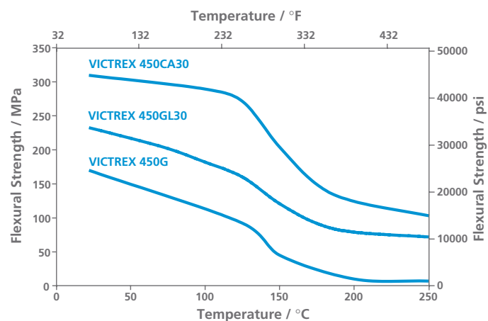
Figure 4: Flexural Strength Versus Temperature for VICTREX PEEK Materials
