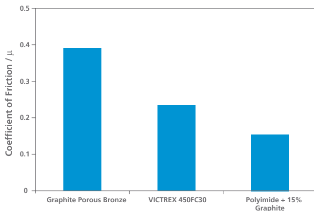
Figure 28: Coefficient of Friction for a Range of Materials at 200°C (390°F), with v = 3 \text{ m s}^{-1} (600 ft \text{min}^{-1} ) and 20 kg (44 lb) Load
