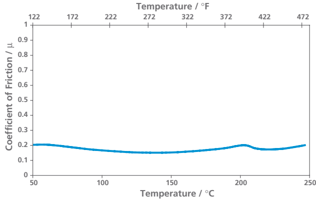
Figure 29: Variation of the Coefficient of Friction with Temperature for VICTREX 450FC30, v = 0.17 \text{ m s}^{-1} (34 ft min -1 ) and 19 kg (41 lb) Load
